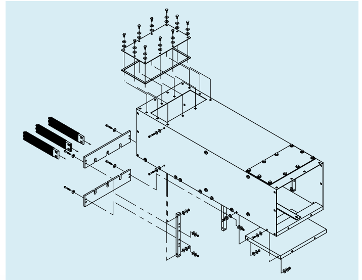
Housing Assembly
